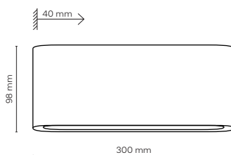
18186 / ARWENA LED INTEGRATED LED
