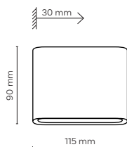
18184 / ARWENA LED INTEGRATED LED
