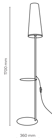
5959 / ZIGN 1 x GU10 / 230V / max 10W / LED AB / ? 1234
