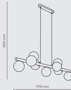
5906 / ESTERA WOOD 9 x G9 / 230V / max 6W / LED KL / 7454
