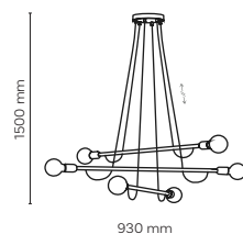
4950 / HELIX WOOD 6 x E27 / 230V / max 15W / LED 4950 4953
