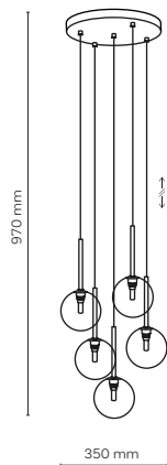
5943 / NILOS 5 x G9 / 230V / max 6W / LED KL / 7525 (ø 120mm)
