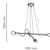
4949 / HELIX WOOD 4 x E27 / 230V / max 15W / LED 4949 4952
